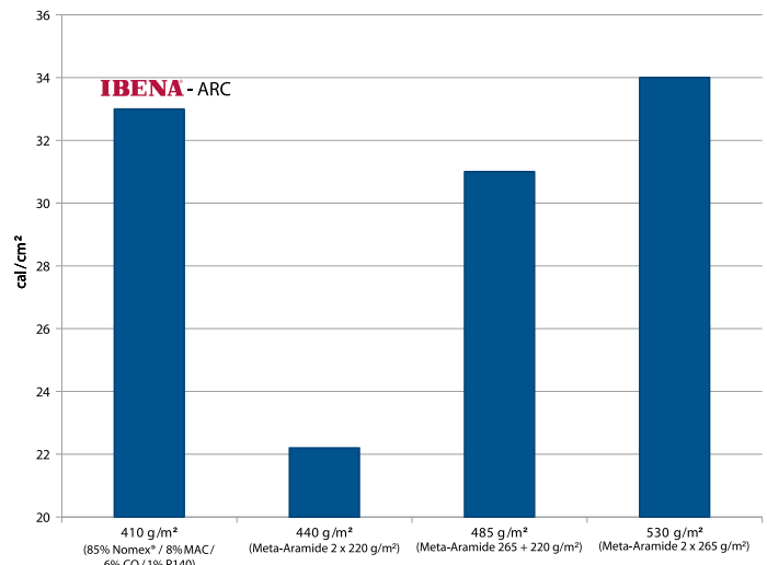
ATPV results of 2-layer systems
